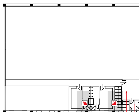
PALESTRA 1° PIANO GYMNASE 1 ER ÉTAGE - GYM FIRST FLOOR
